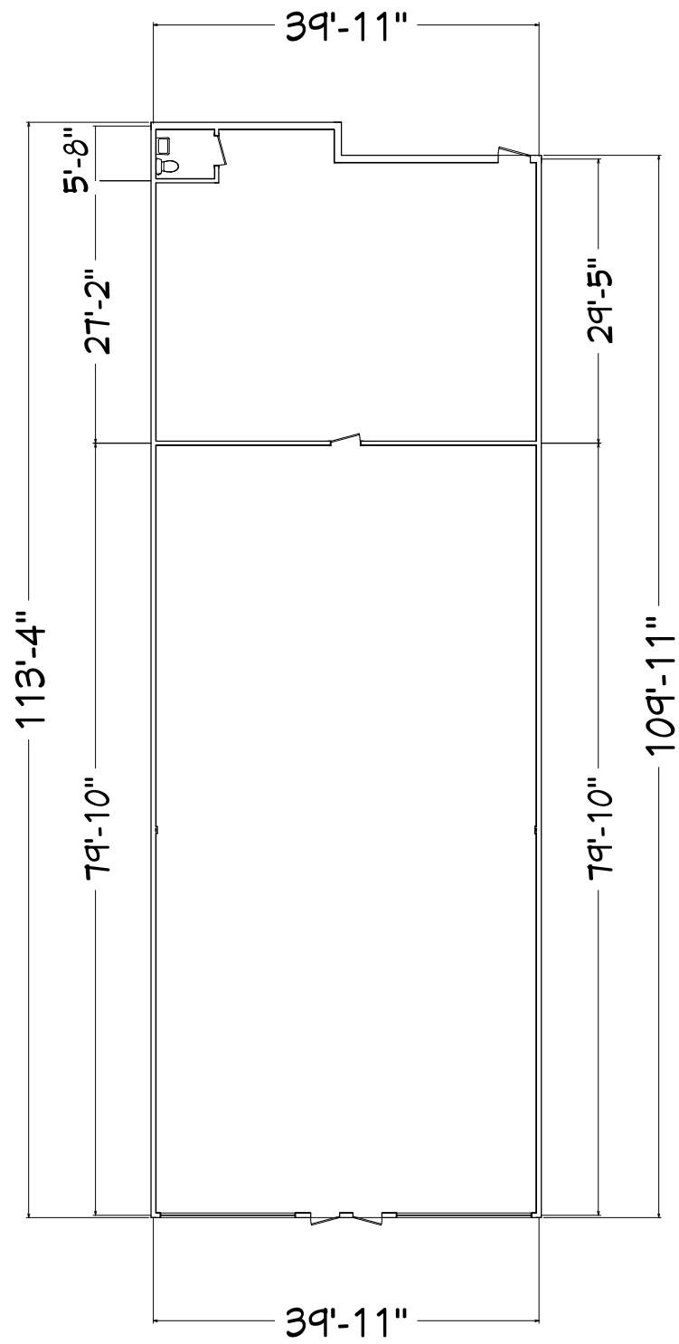
1st Floor
