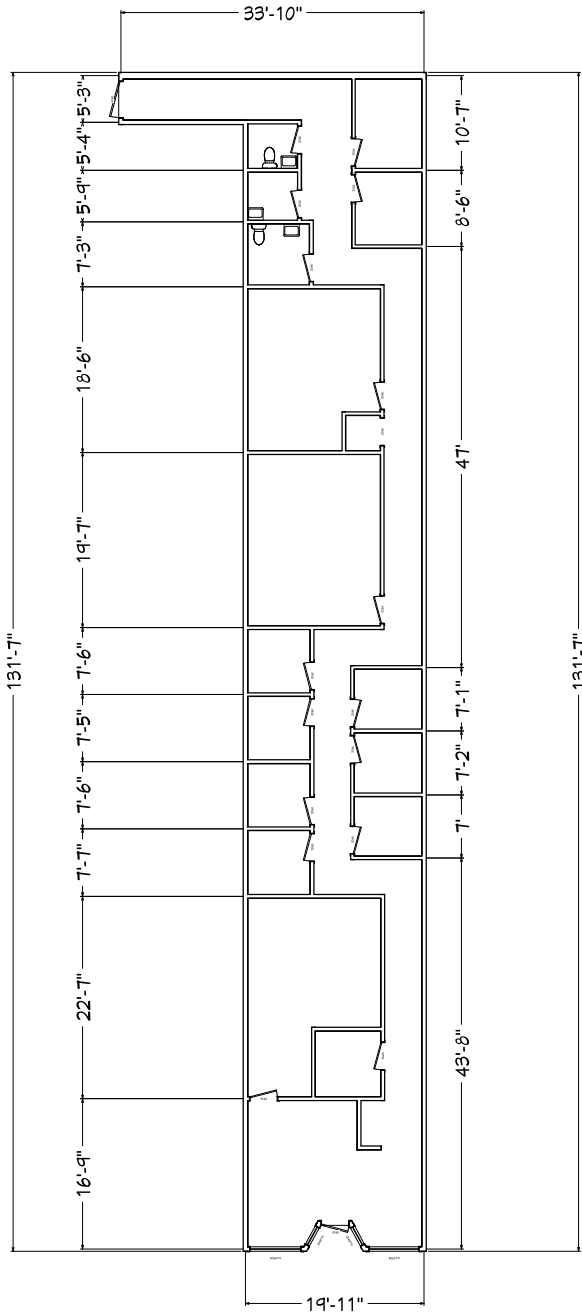
1st Floor
