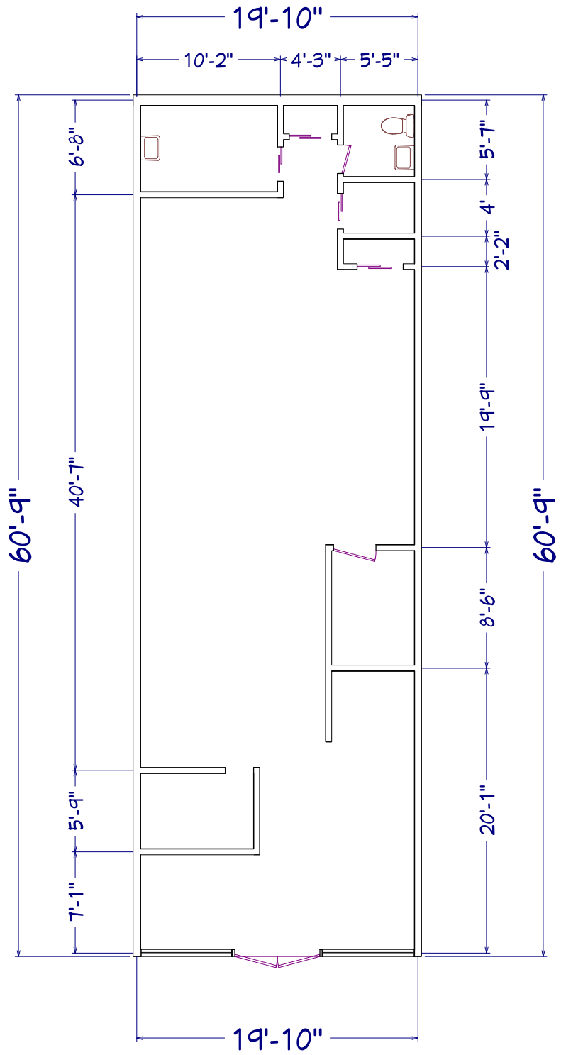
1st Floor
