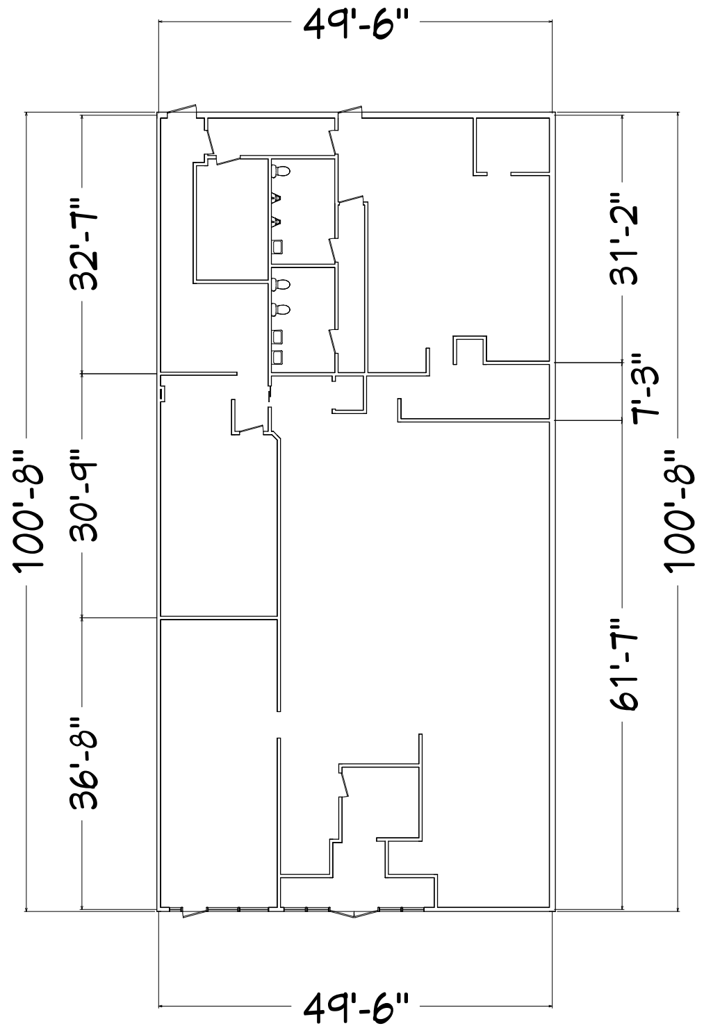
1st Floor
