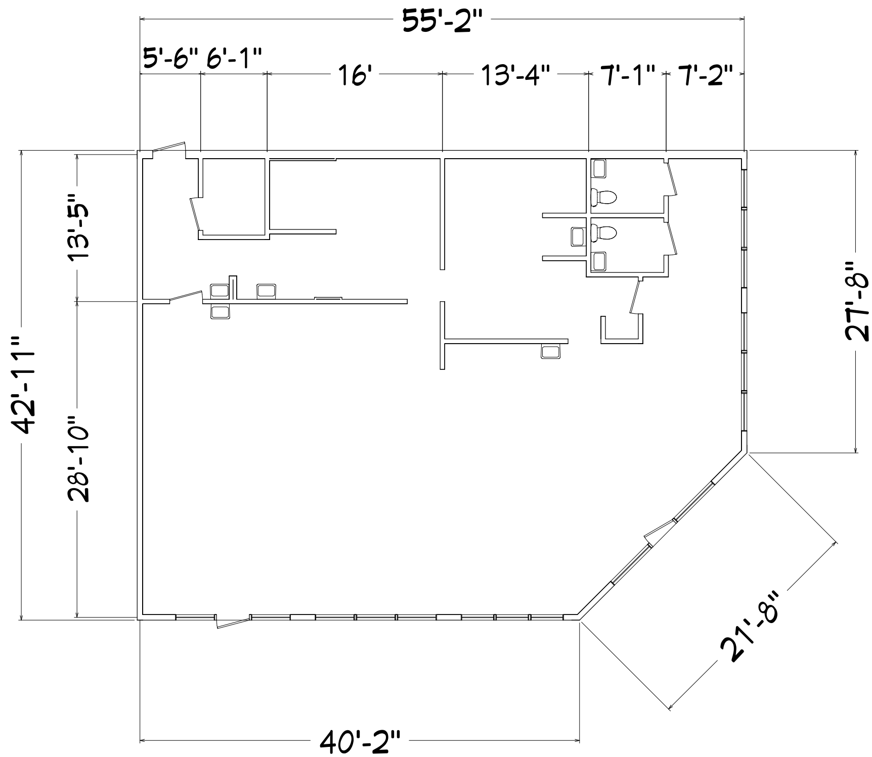
1st Floor
