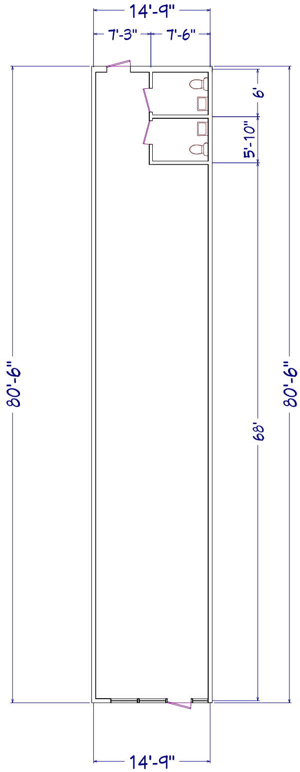
1st Floor
