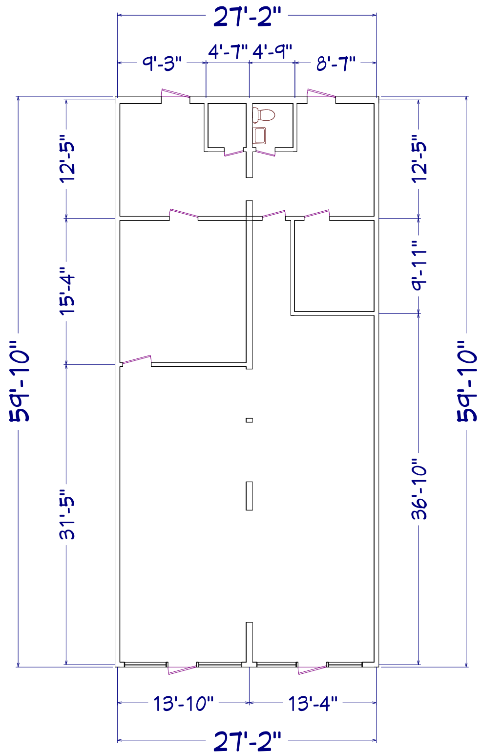
1st Floor
