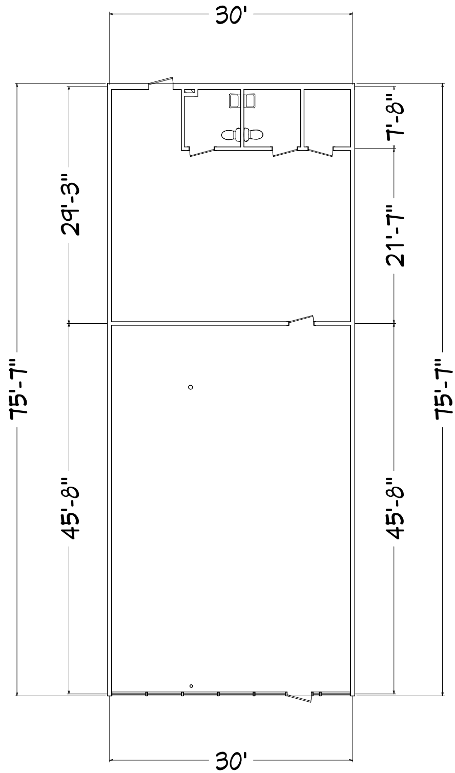
1st Floor
