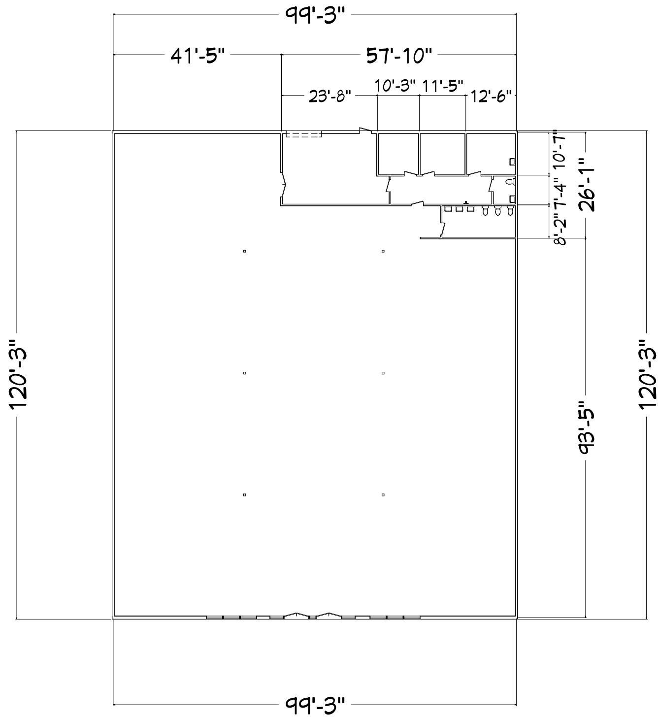
1st Floor
