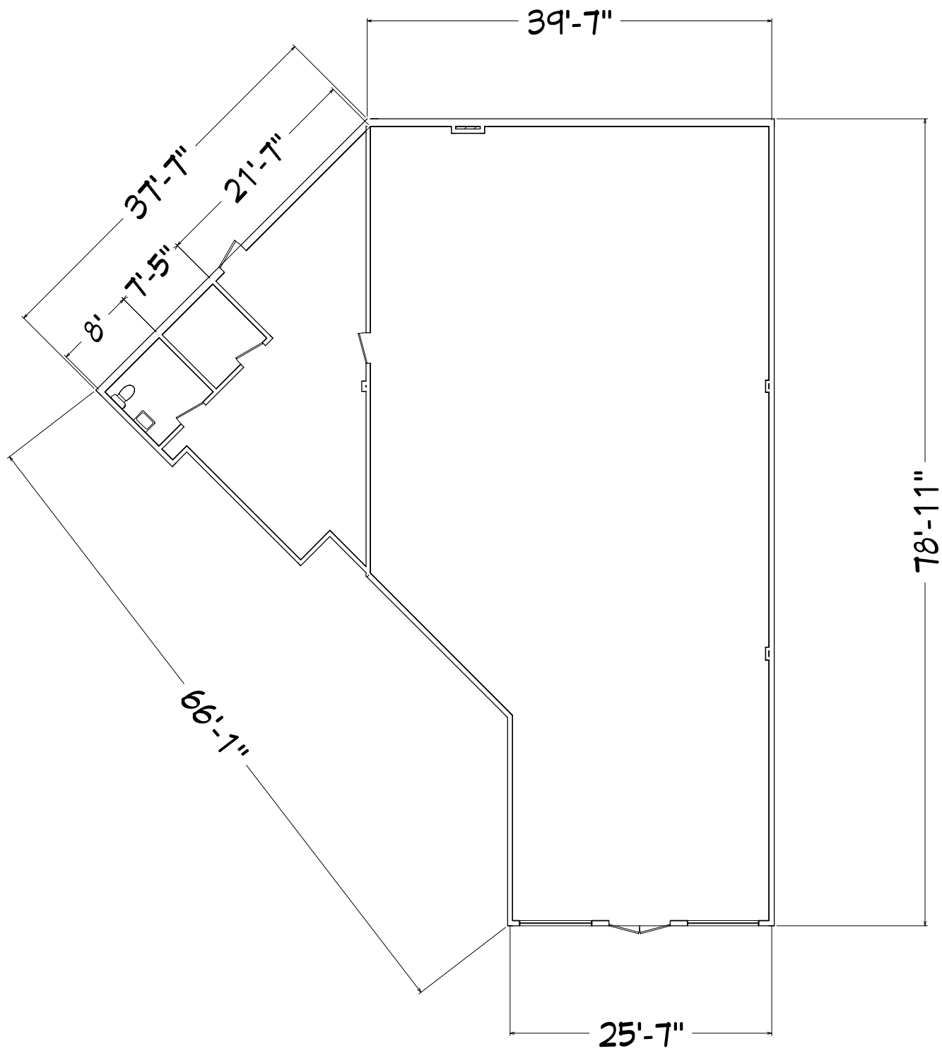
1st Floor
