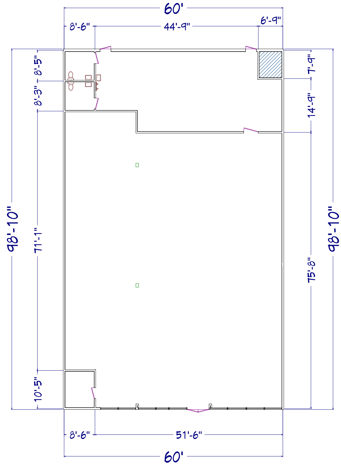
1st Floor
