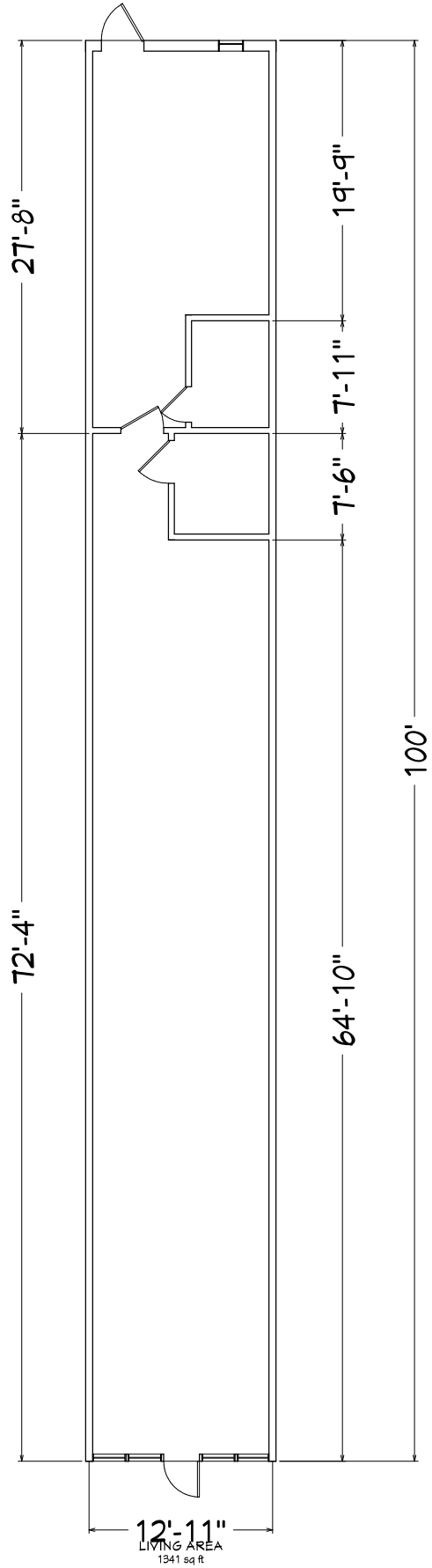
1st Floor
